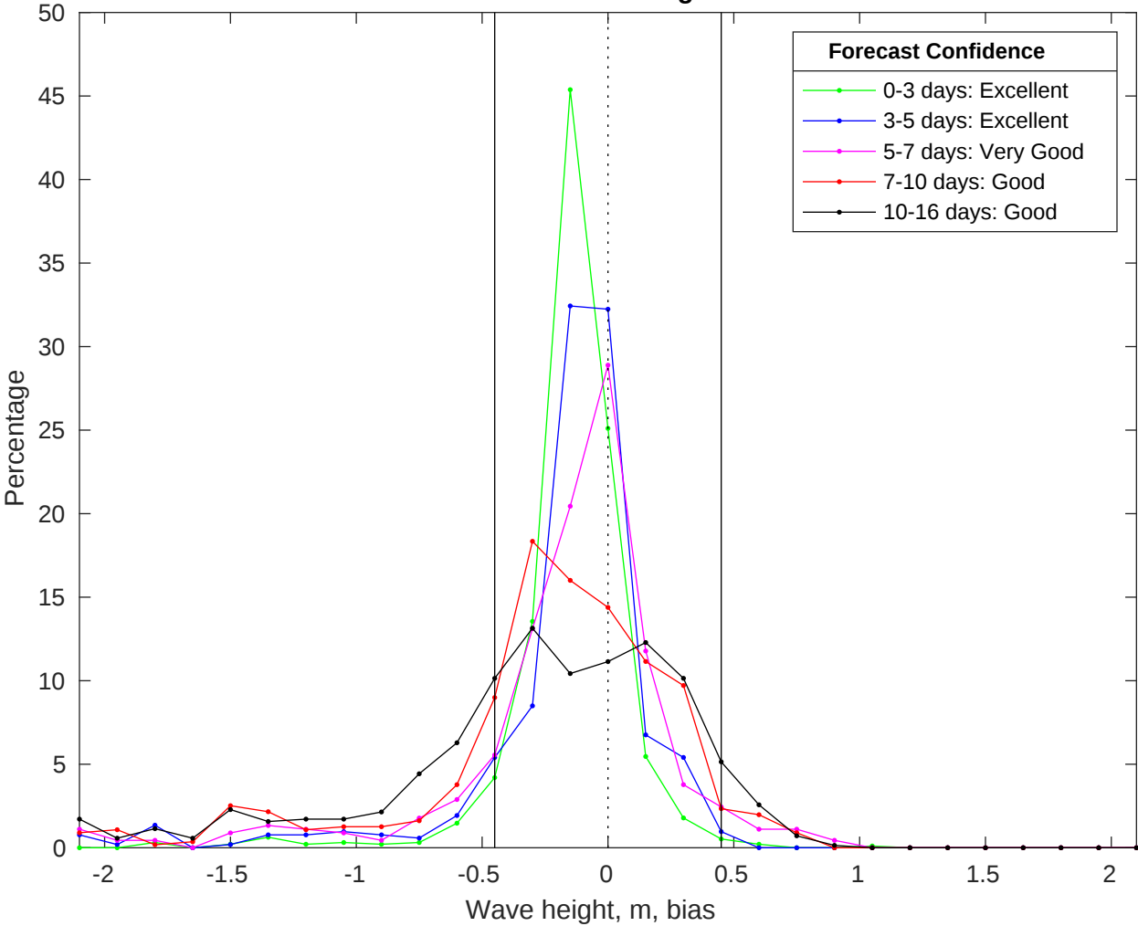
NDBC 41013 vs GFS Waves Bias Histogram: 09-Jul-2025
