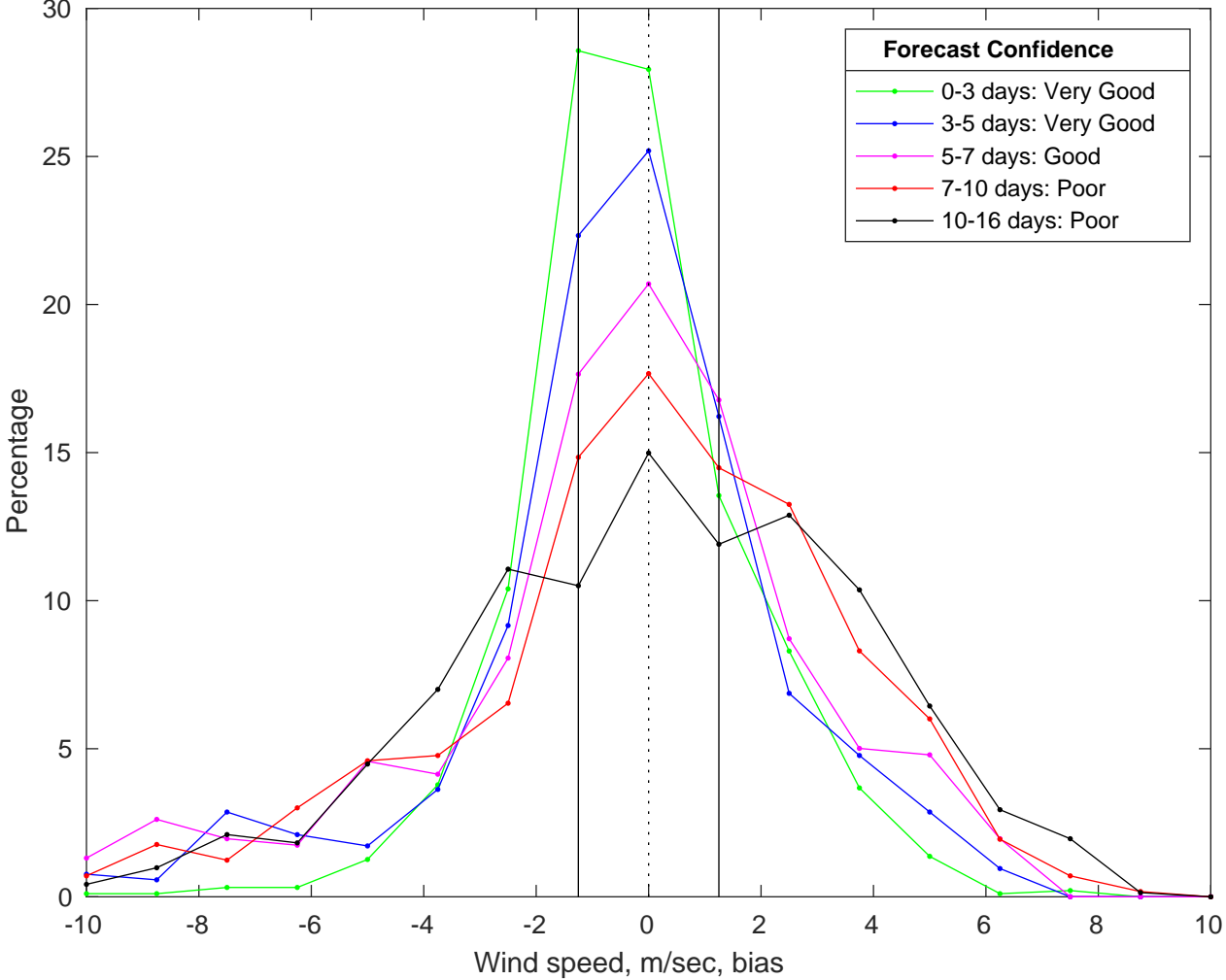
NDBC 41013 vs GFS Winds Bias Histogram: 09-Jul-2025
