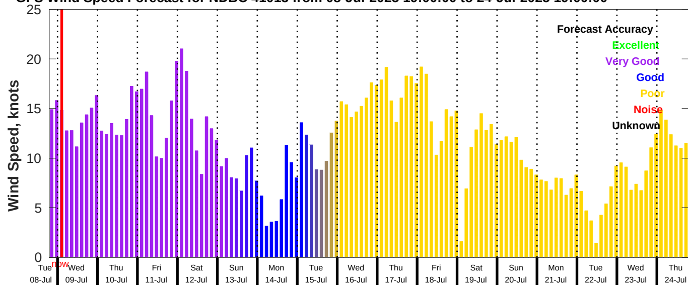
GFS Wind Speed Forecast for NDBC 41013 from 08-Jul-2025 19:00:00 to 24-Jul-2025 19:00:00
