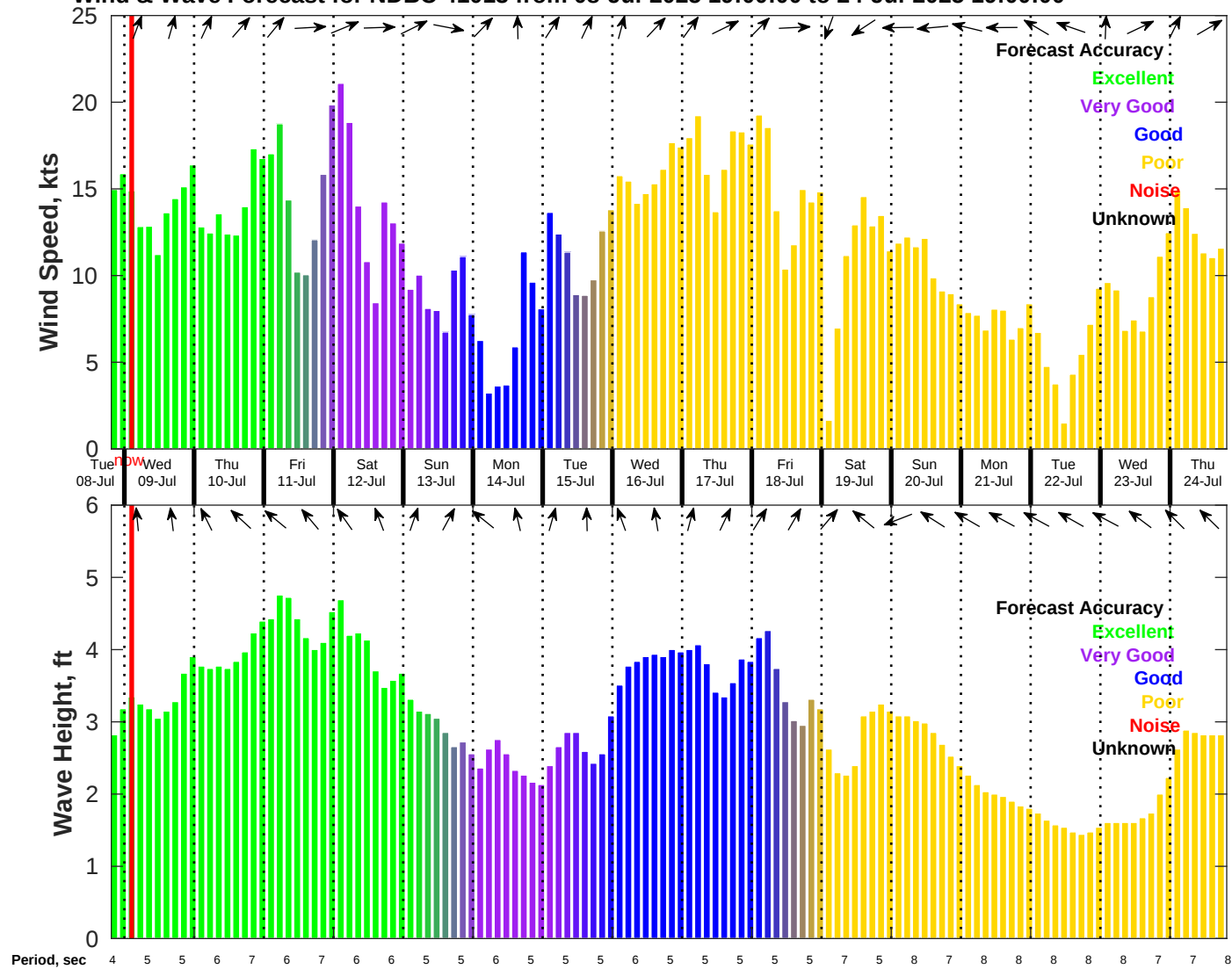
Wind & Wave Forecast for NDBC 41013 from 08-Jul-2025 19:00:00 to 24-Jul-2025 19:00:00
