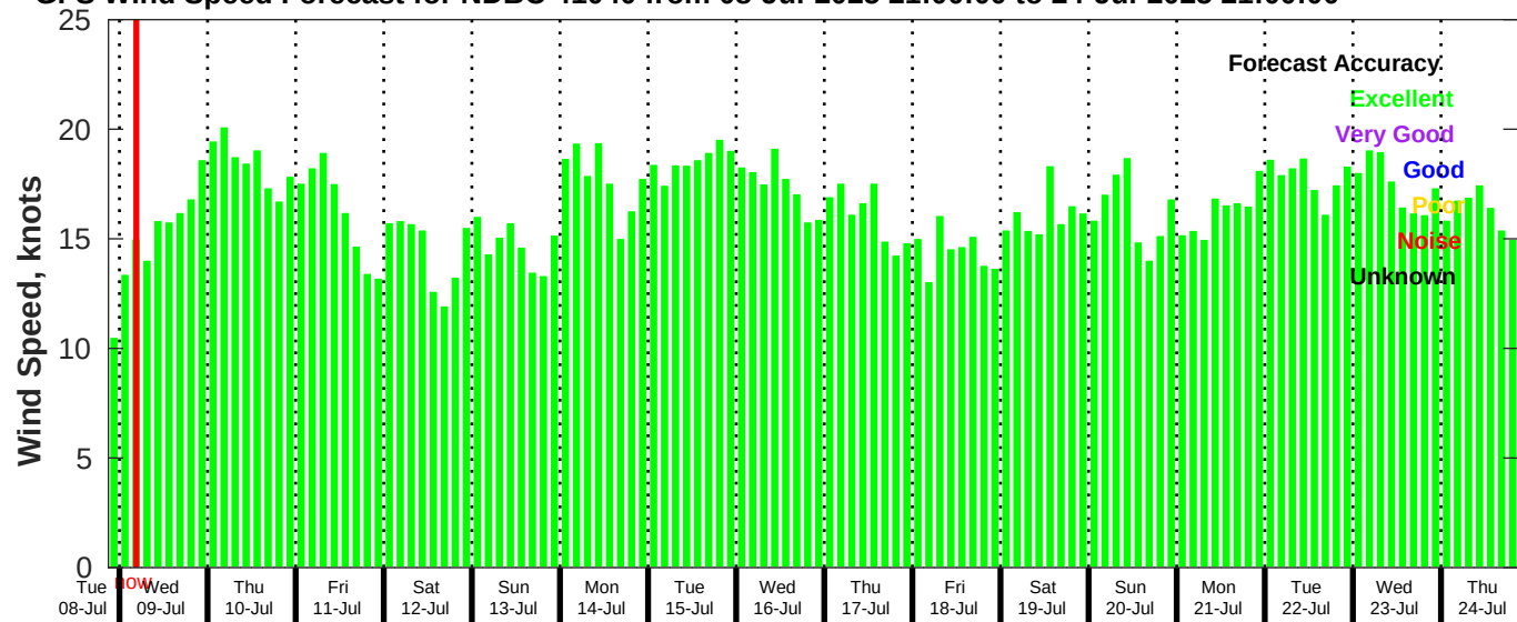
GFS Wind Speed Forecast for NDBC 41040 from 08-Jul-2025 21:00:00 to 24-Jul-2025 21:00:00
