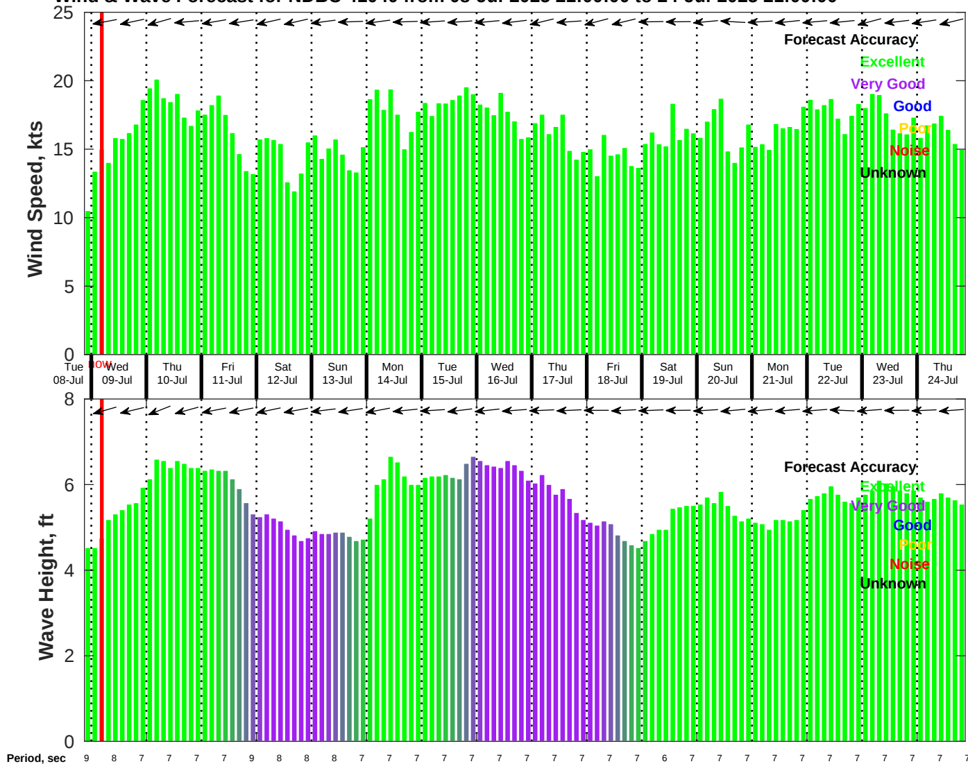
Wind & Wave Forecast for NDBC 41040 from 08-Jul-2025 21:00:00 to 24-Jul-2025 21:00:00
