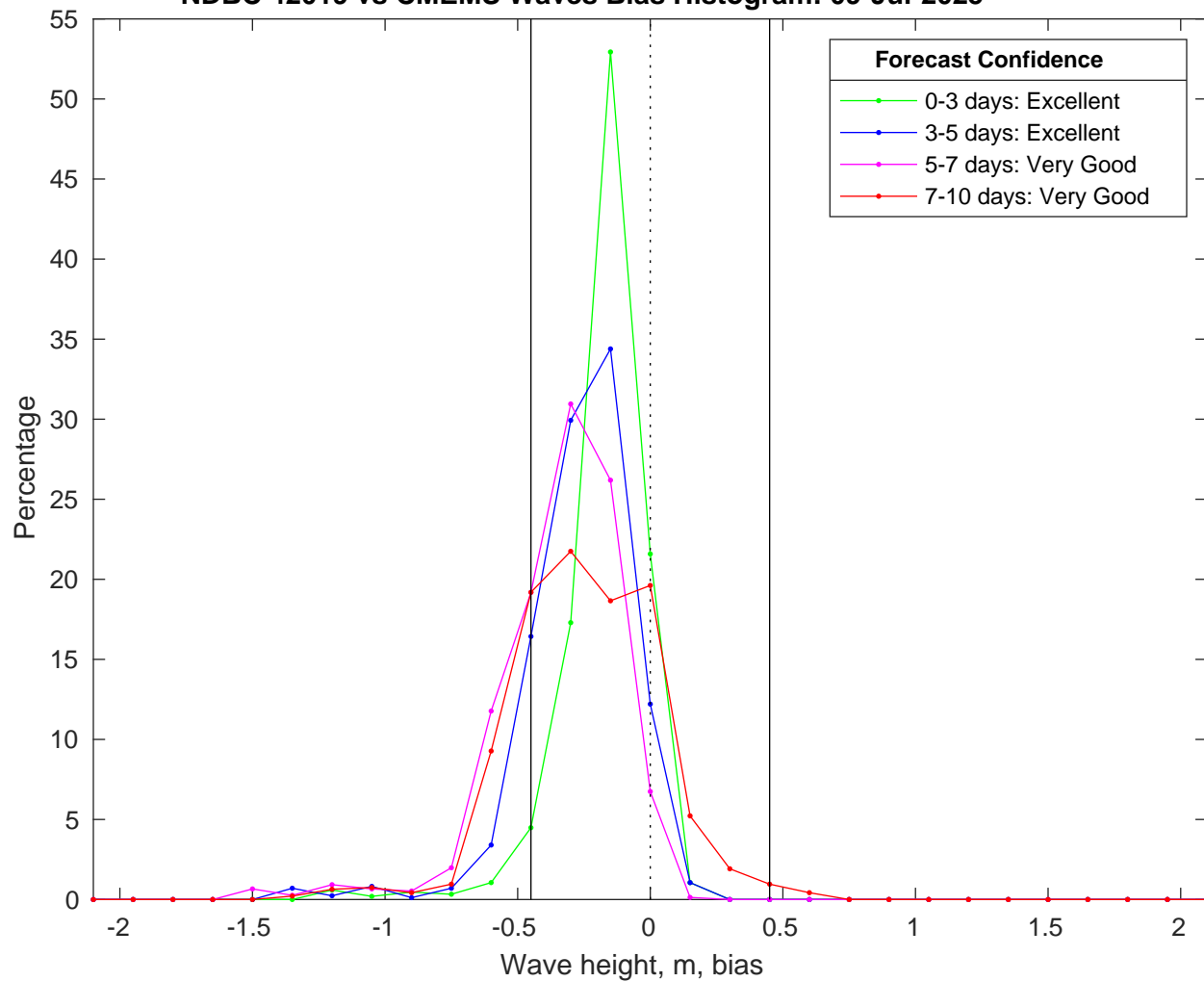
NDBC 42019 vs CMEMS Waves Bias Histogram: 09-Jul-2025
