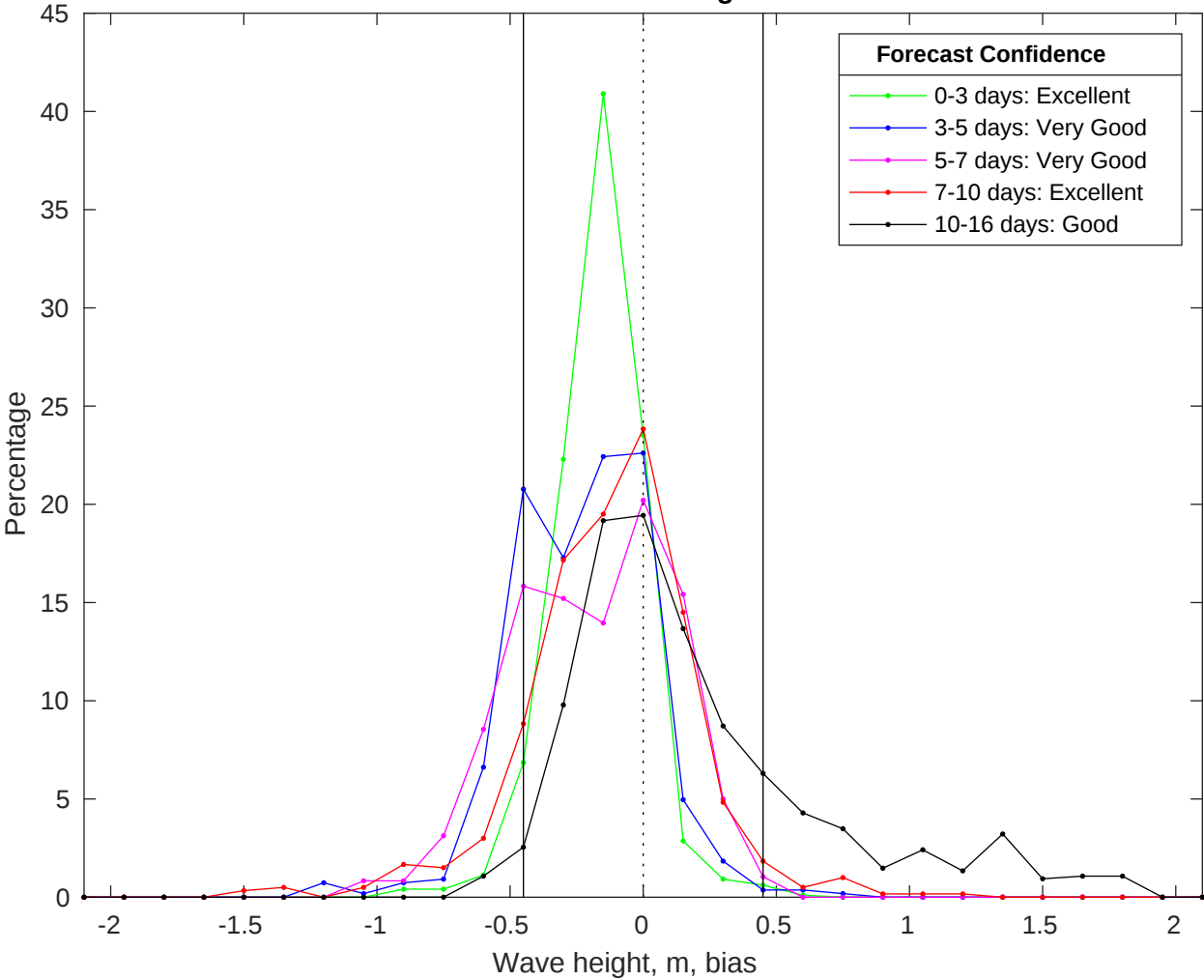
NDBC 42019 vs GFS Waves Bias Histogram: 09-Jul-2025
