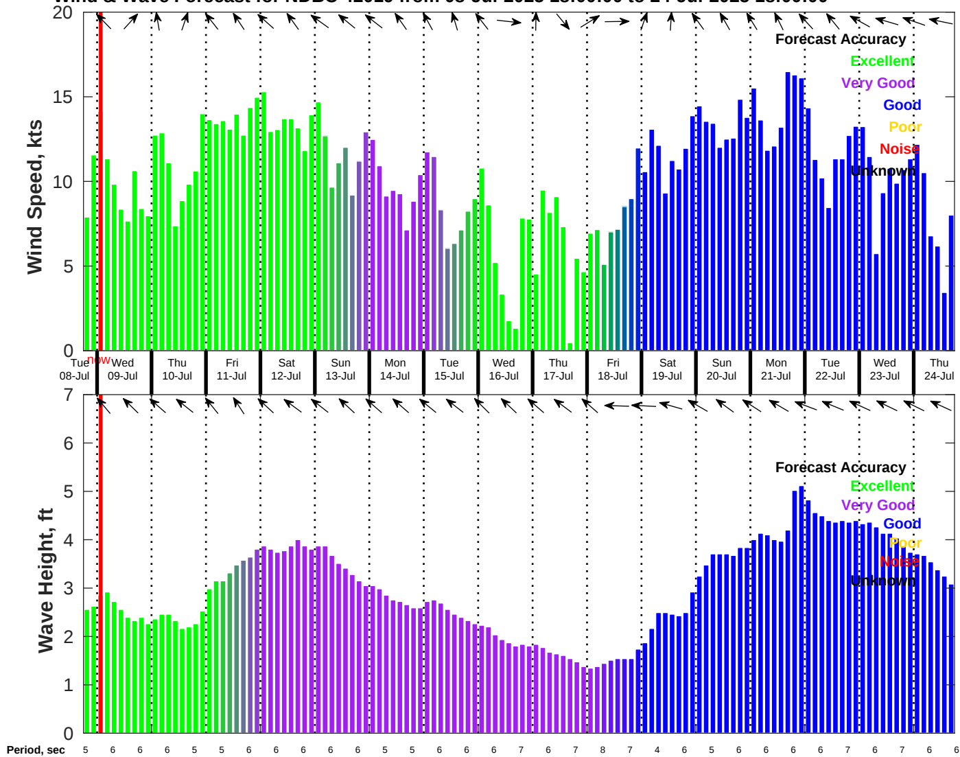
Wind & Wave Forecast for NDBC 42019 from 08-Jul-2025 18:00:00 to 24-Jul-2025 18:00:00
