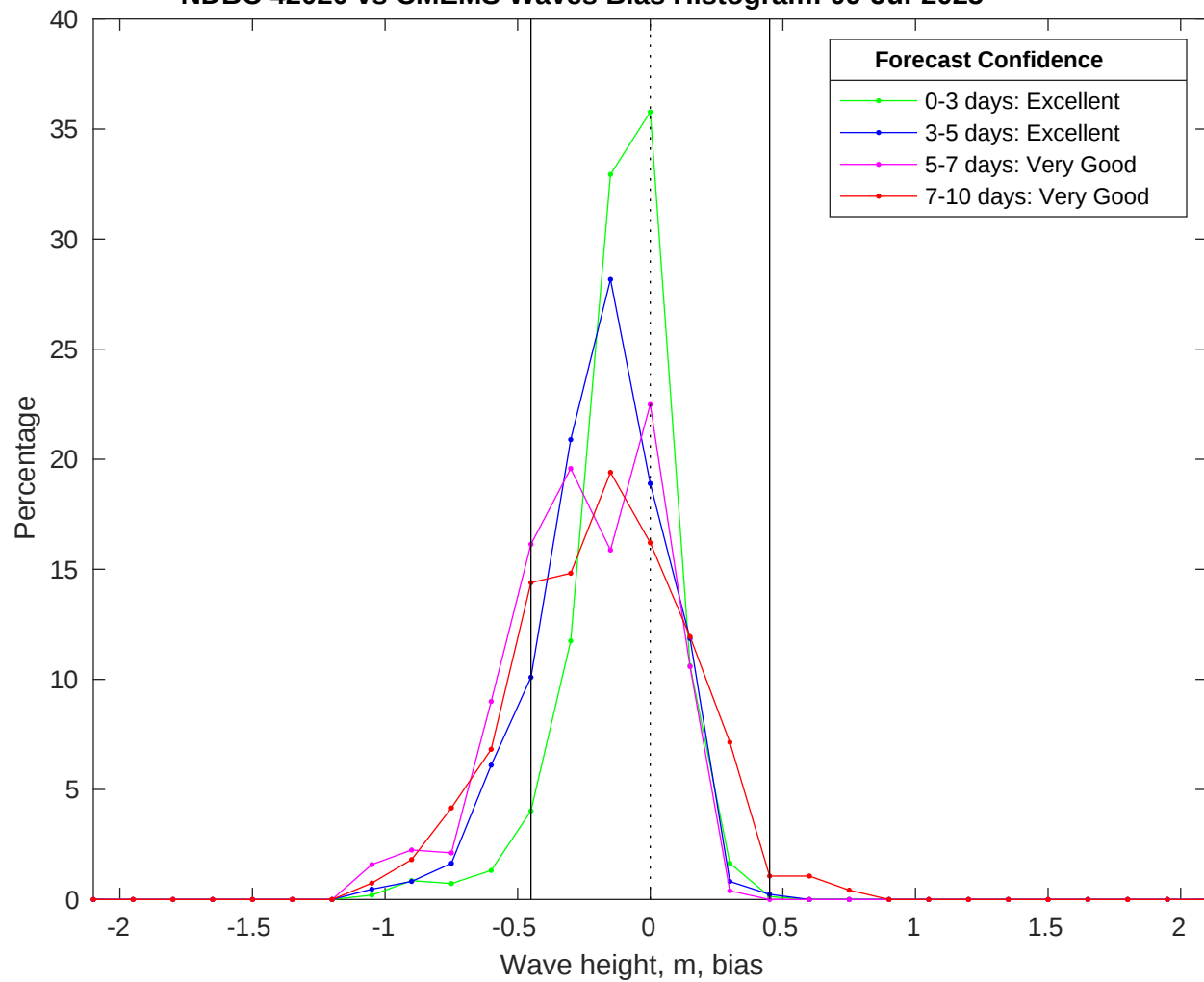
NDBC 42020 vs CMEMS Waves Bias Histogram: 09-Jul-2025
