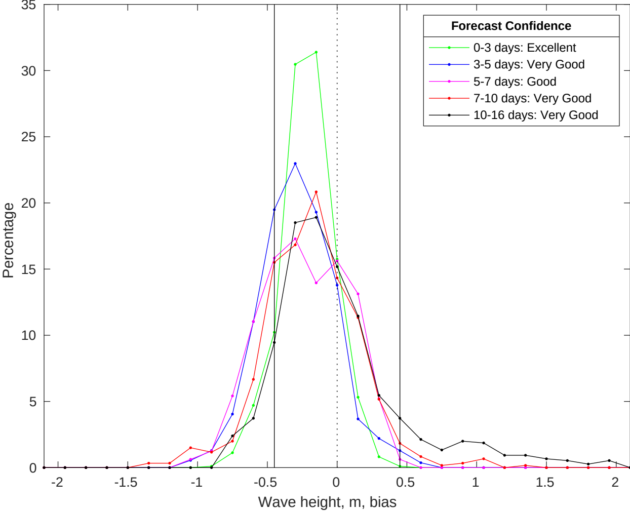
NDBC 42020 vs GFS Waves Bias Histogram: 09-Jul-2025
