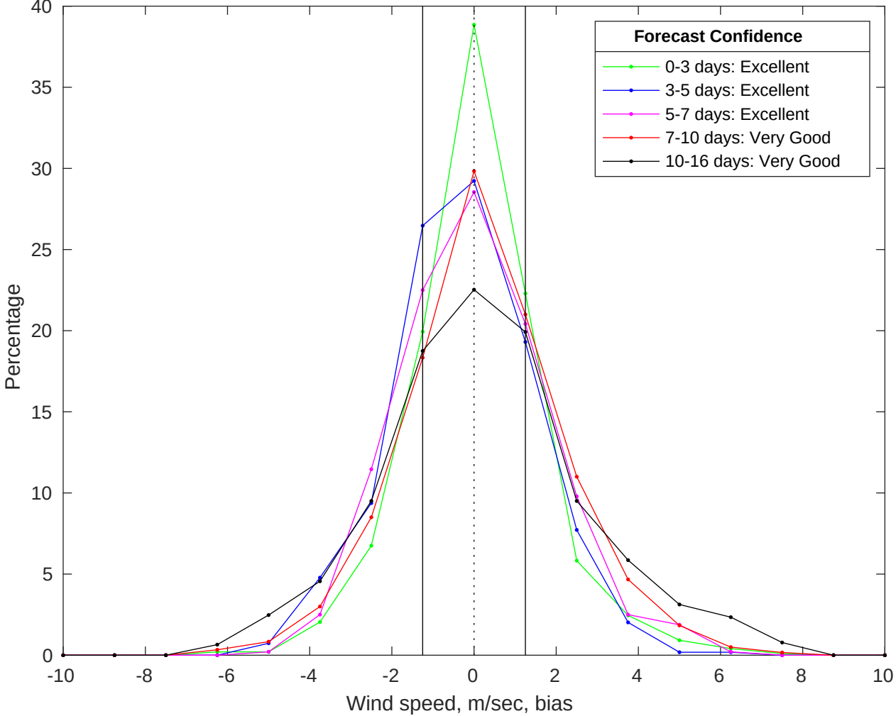
NDBC 42020 vs GFS Winds Bias Histogram: 09-Jul-2025
