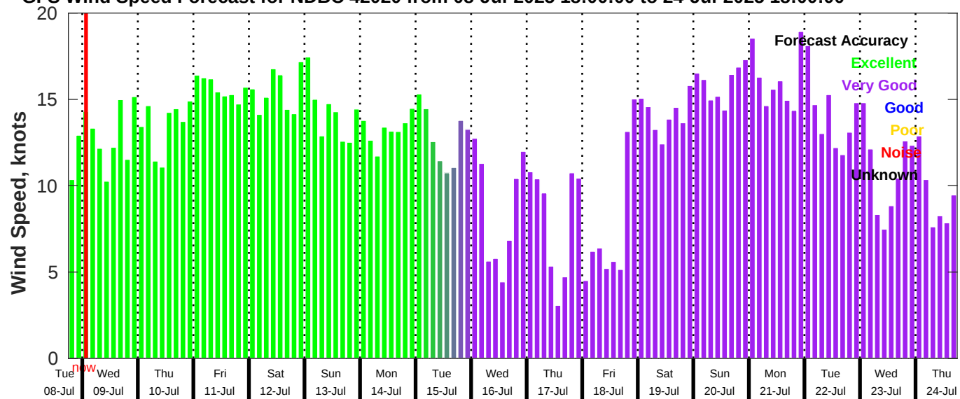
GFS Wind Speed Forecast for NDBC 42020 from 08-Jul-2025 18:00:00 to 24-Jul-2025 18:00:00
