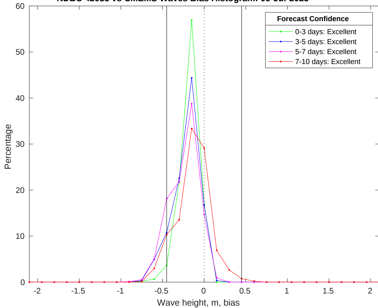
NDBC 42035 vs CMEMS Waves Bias Histogram: 09-Jul-2025
