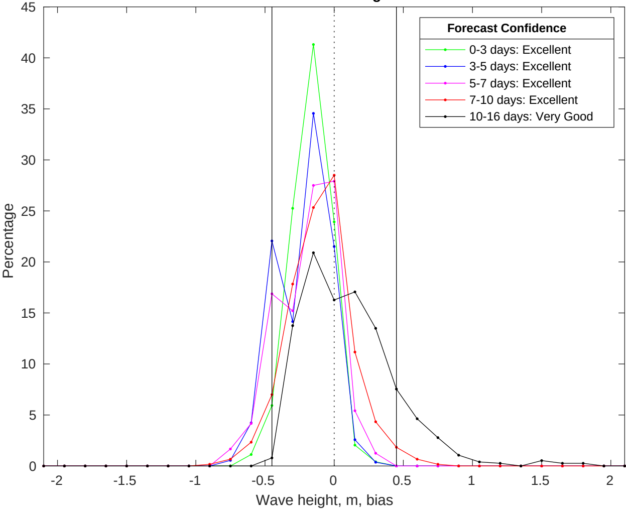
NDBC 42035 vs GFS Waves Bias Histogram: 09-Jul-2025
