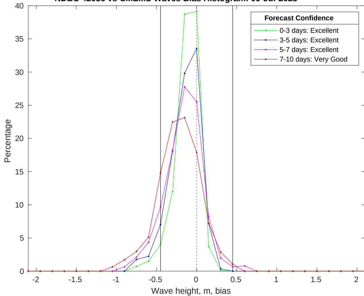
NDBC 42036 vs CMEMS Waves Bias Histogram: 09-Jul-2025
