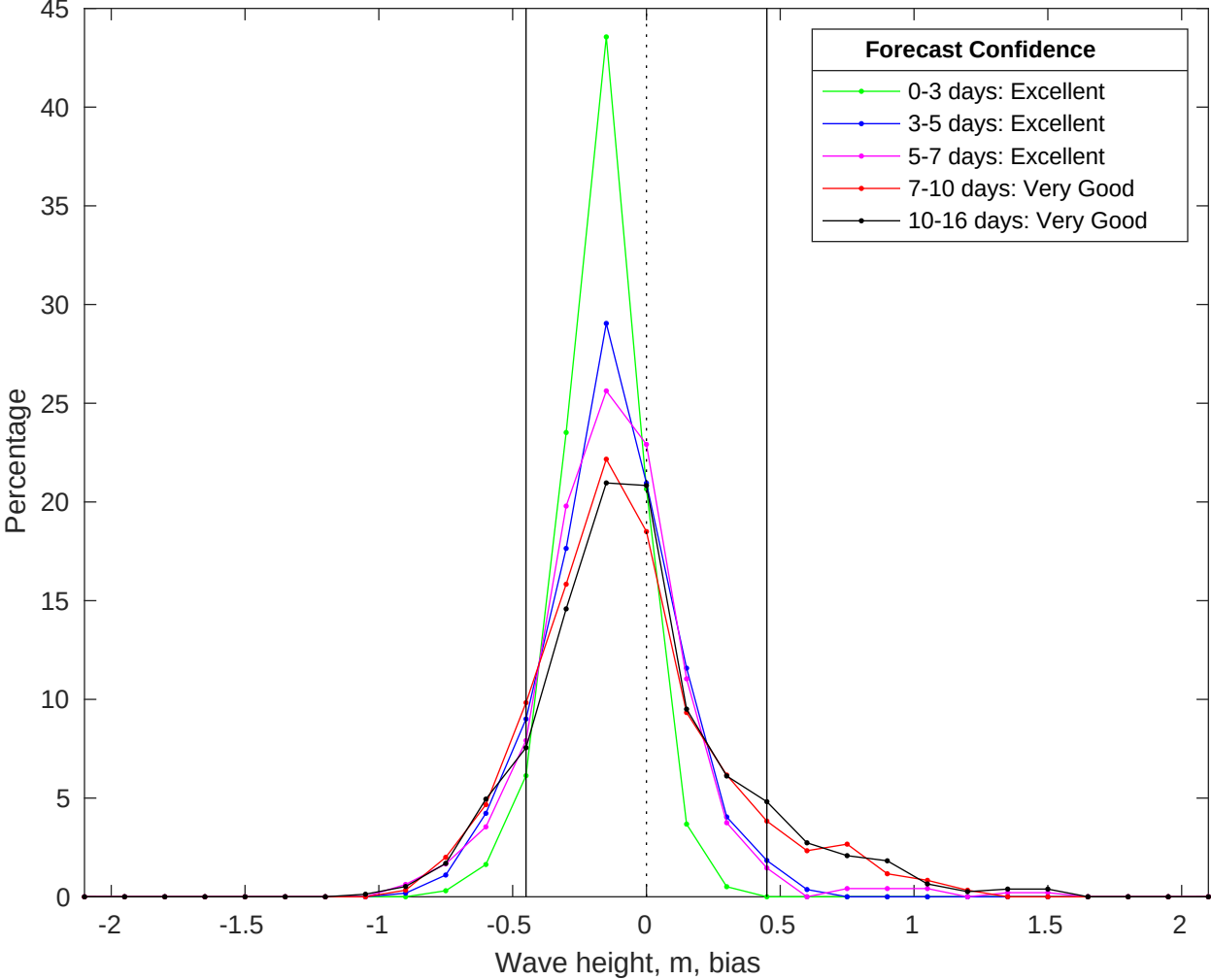
NDBC 42036 vs GFS Waves Bias Histogram: 09-Jul-2025
