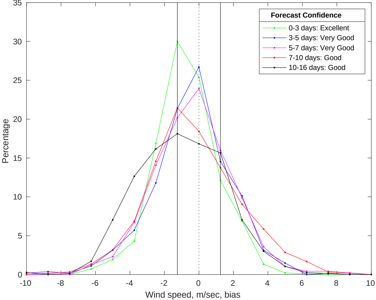
NDBC 42036 vs GFS Winds Bias Histogram: 09-Jul-2025
