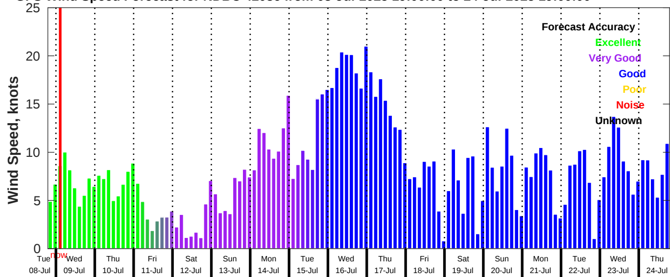
GFS Wind Speed Forecast for NDBC 42036 from 08-Jul-2025 19:00:00 to 24-Jul-2025 19:00:00
