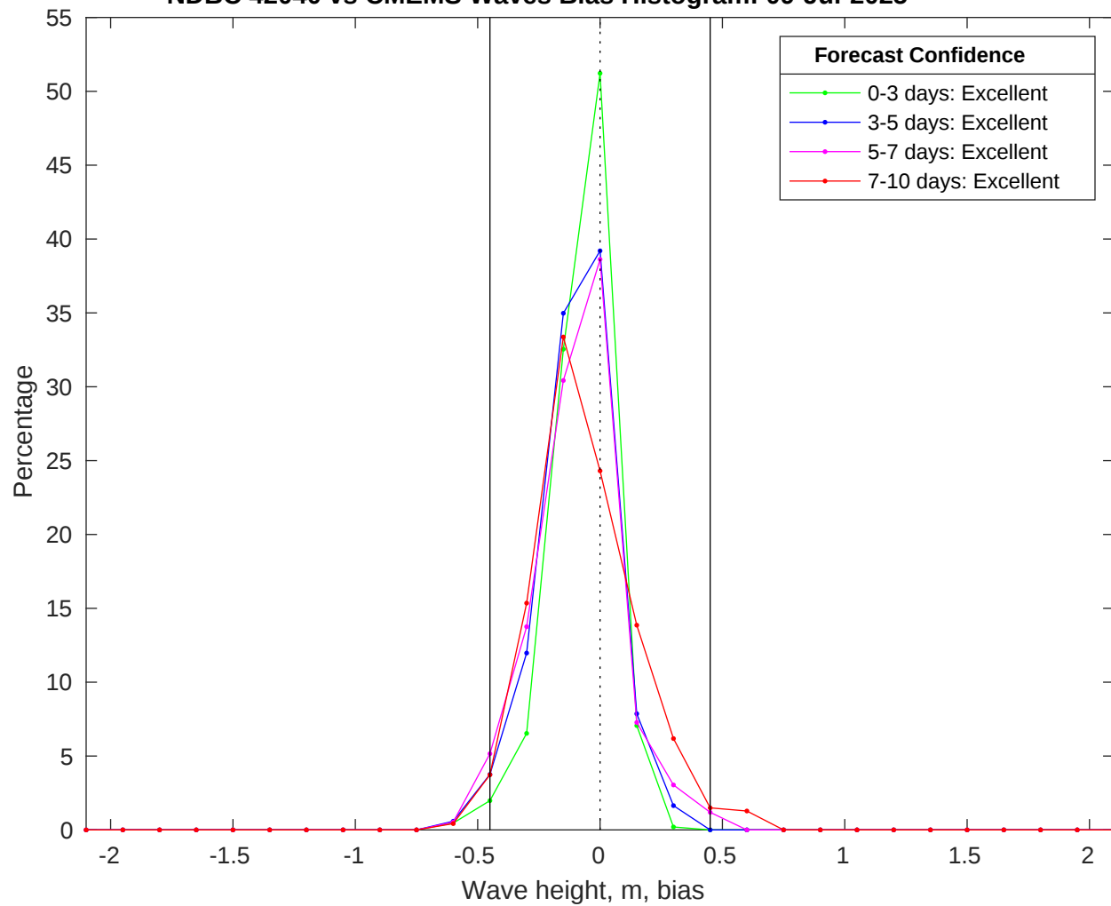
NDBC 42040 vs CMEMS Waves Bias Histogram: 09-Jul-2025
