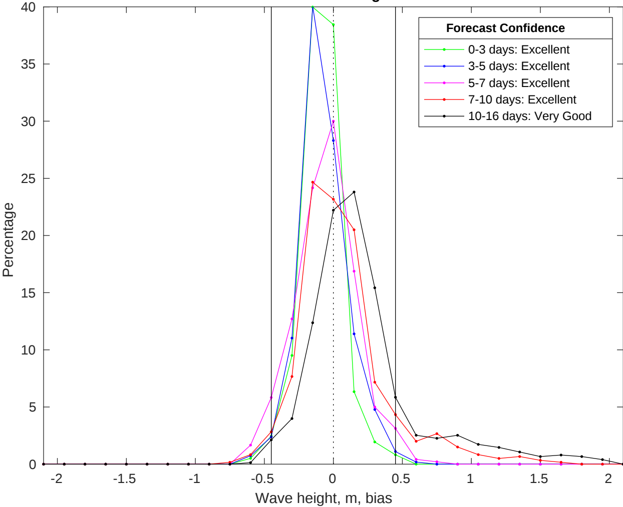
NDBC 42040 vs GFS Waves Bias Histogram: 09-Jul-2025
