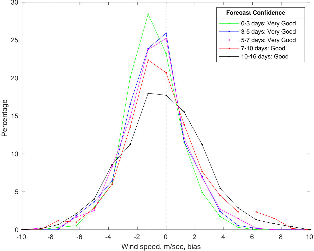
NDBC 42040 vs GFS Winds Bias Histogram: 09-Jul-2025
