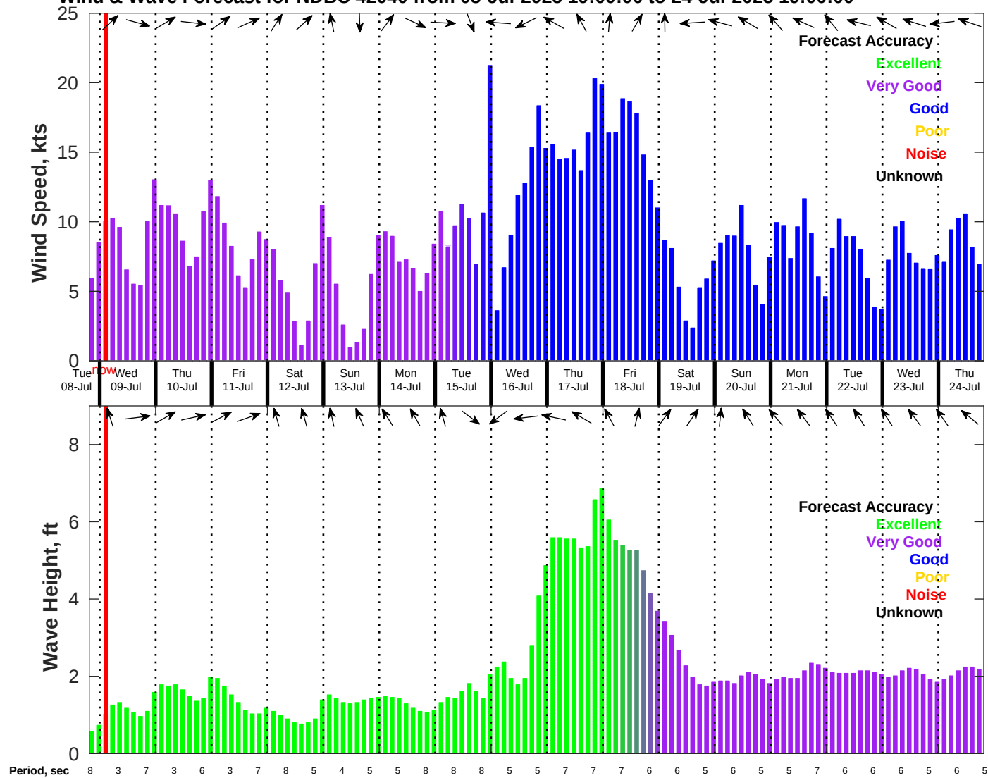
Wind & Wave Forecast for NDBC 42040 from 08-Jul-2025 19:00:00 to 24-Jul-2025 19:00:00
