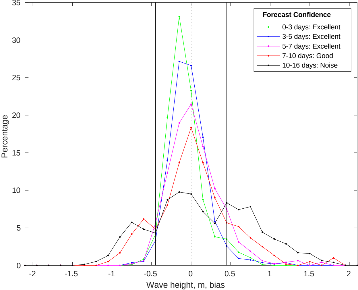
NDBC 46011 vs GFS Waves Bias Histogram: 09-Jul-2025
