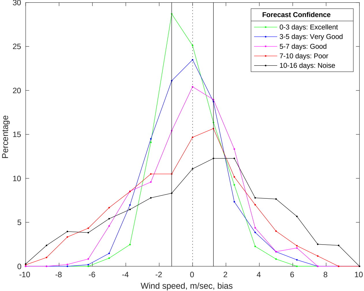
NDBC 46011 vs GFS Winds Bias Histogram: 09-Jul-2025
