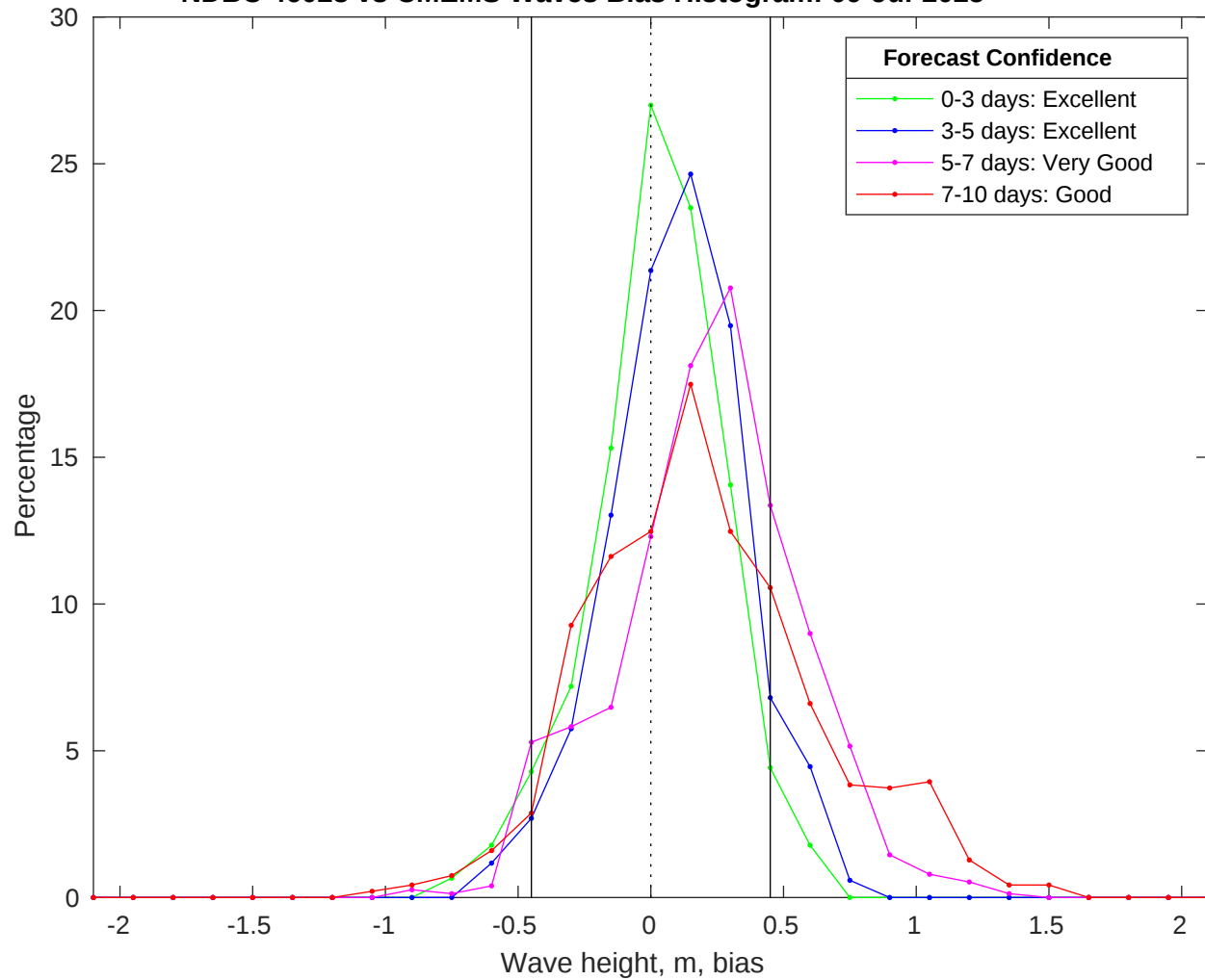
NDBC 46028 vs CMEMS Waves Bias Histogram: 09-Jul-2025
