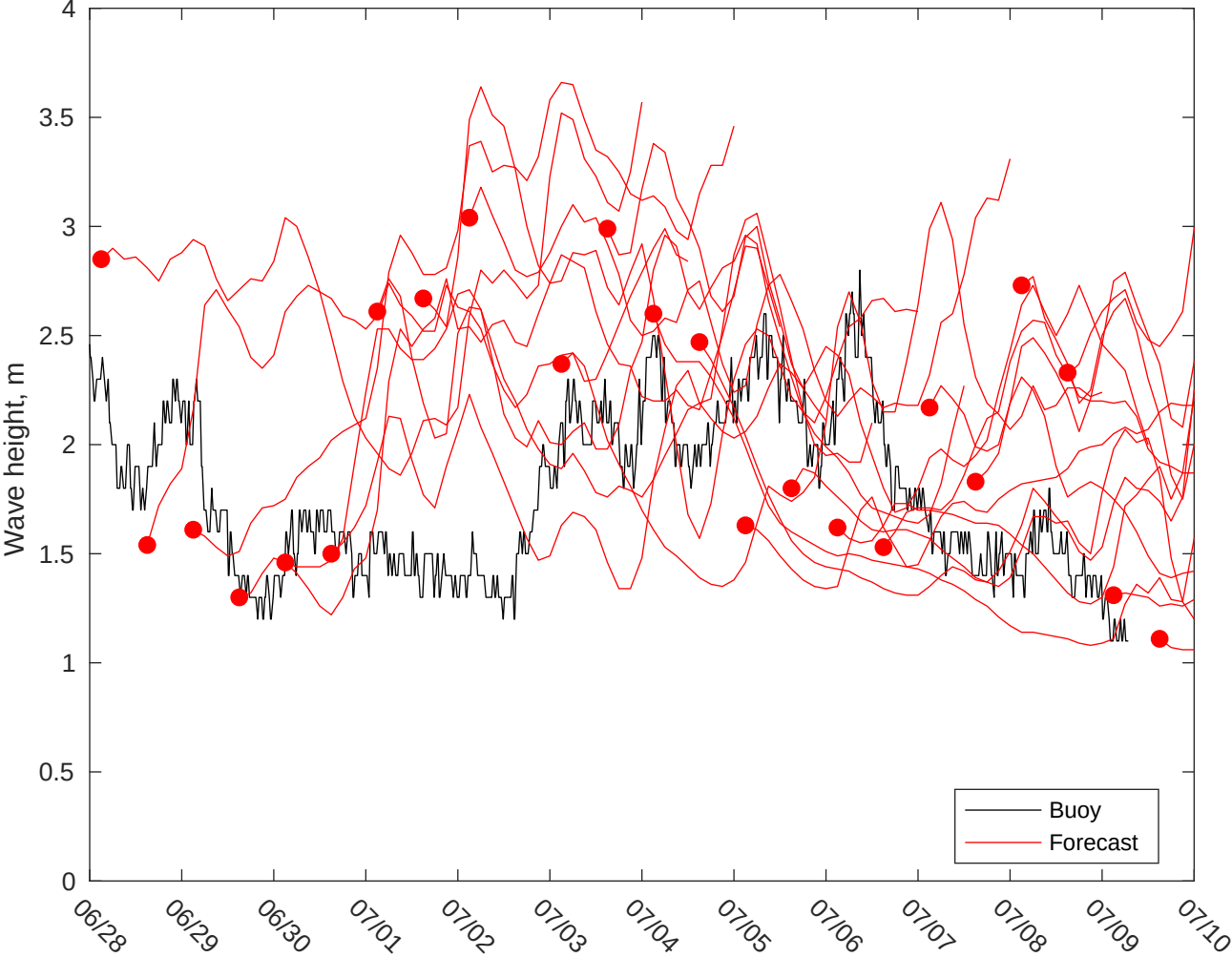
NDBC 46028 vs GFS Waves: 10 to 16 day forecast
