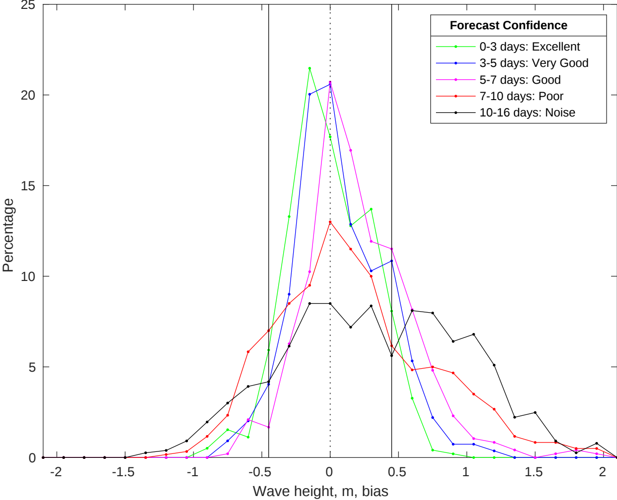
NDBC 46028 vs GFS Waves Bias Histogram: 09-Jul-2025
