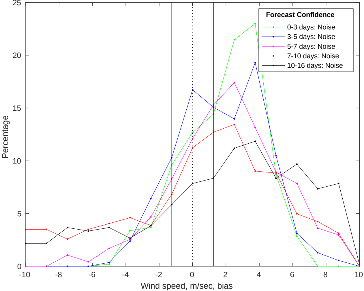
NDBC 46028 vs GFS Winds Bias Histogram: 09-Jul-2025
