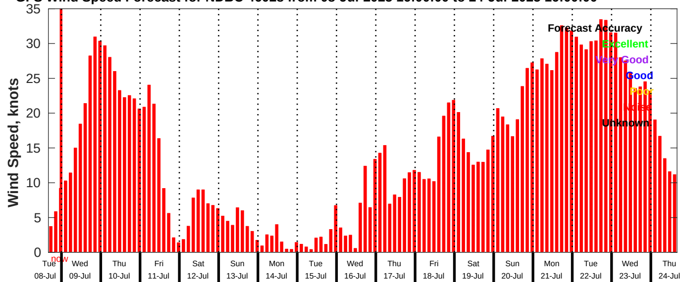
GFS Wind Speed Forecast for NDBC 46028 from 08-Jul-2025 16:00:00 to 24-Jul-2025 16:00:00
