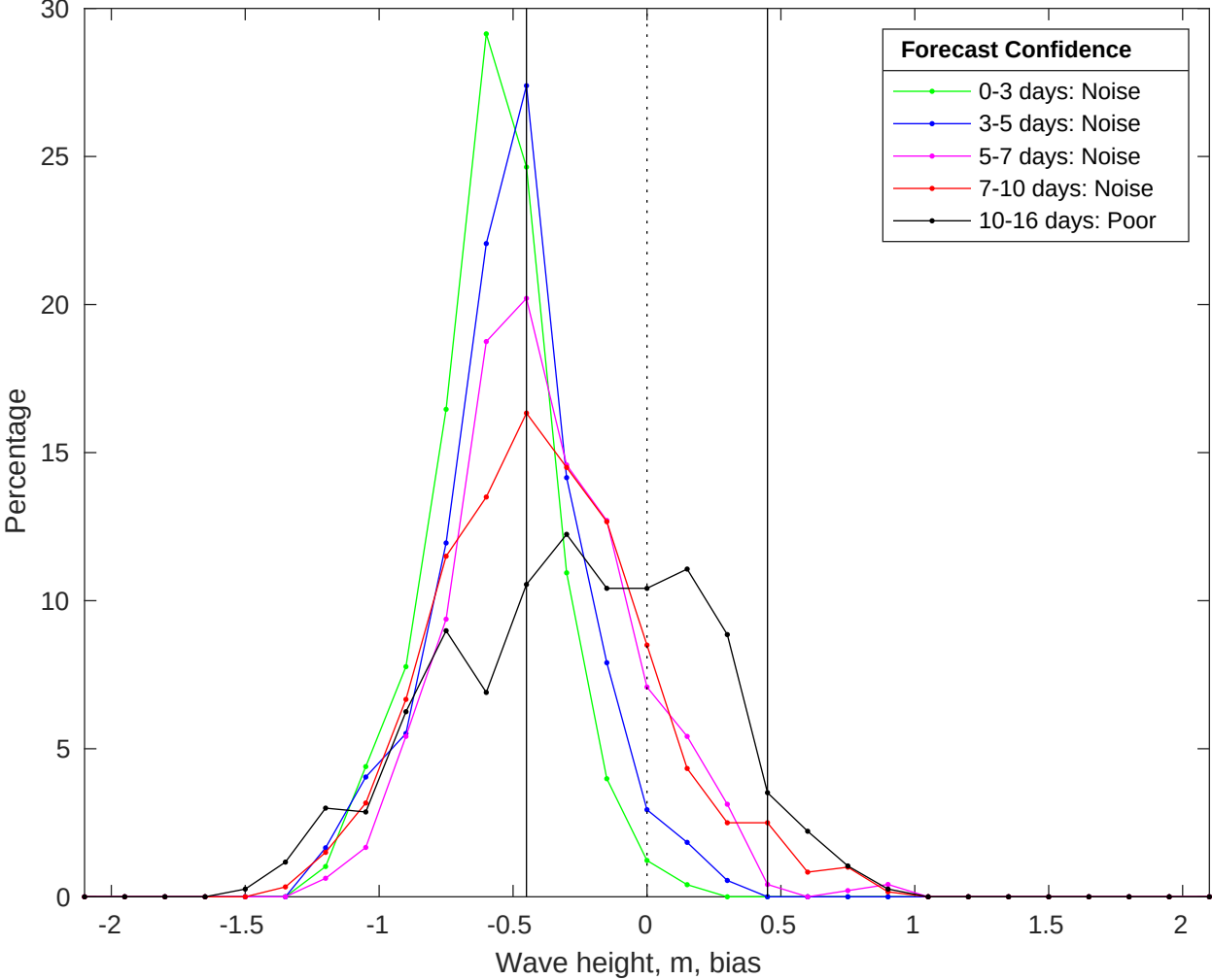
NDBC 46054 vs GFS Waves Bias Histogram: 09-Jul-2025
