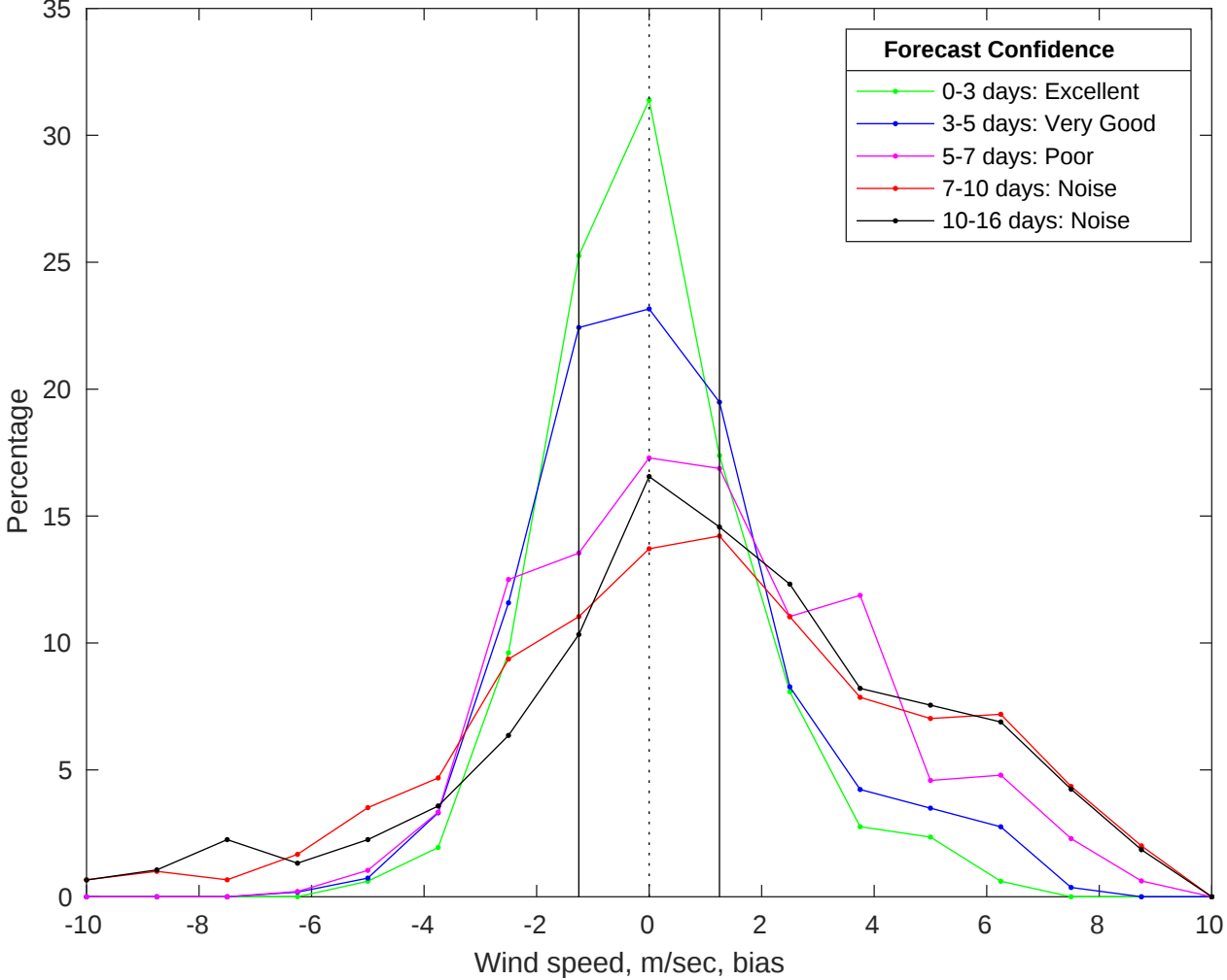
NDBC 46054 vs GFS Winds Bias Histogram: 09-Jul-2025
