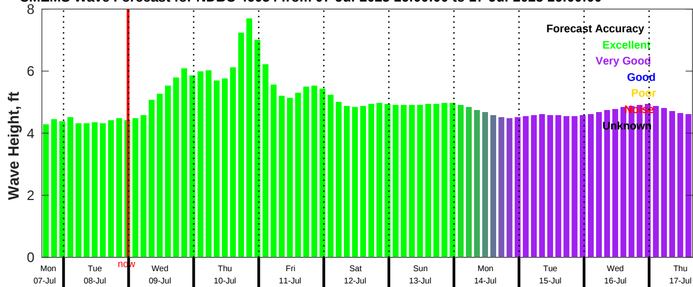
CMEMS Wave Forecast for NDBC 46054 from 07-Jul-2025 16:00:00 to 17-Jul-2025 16:00:00
