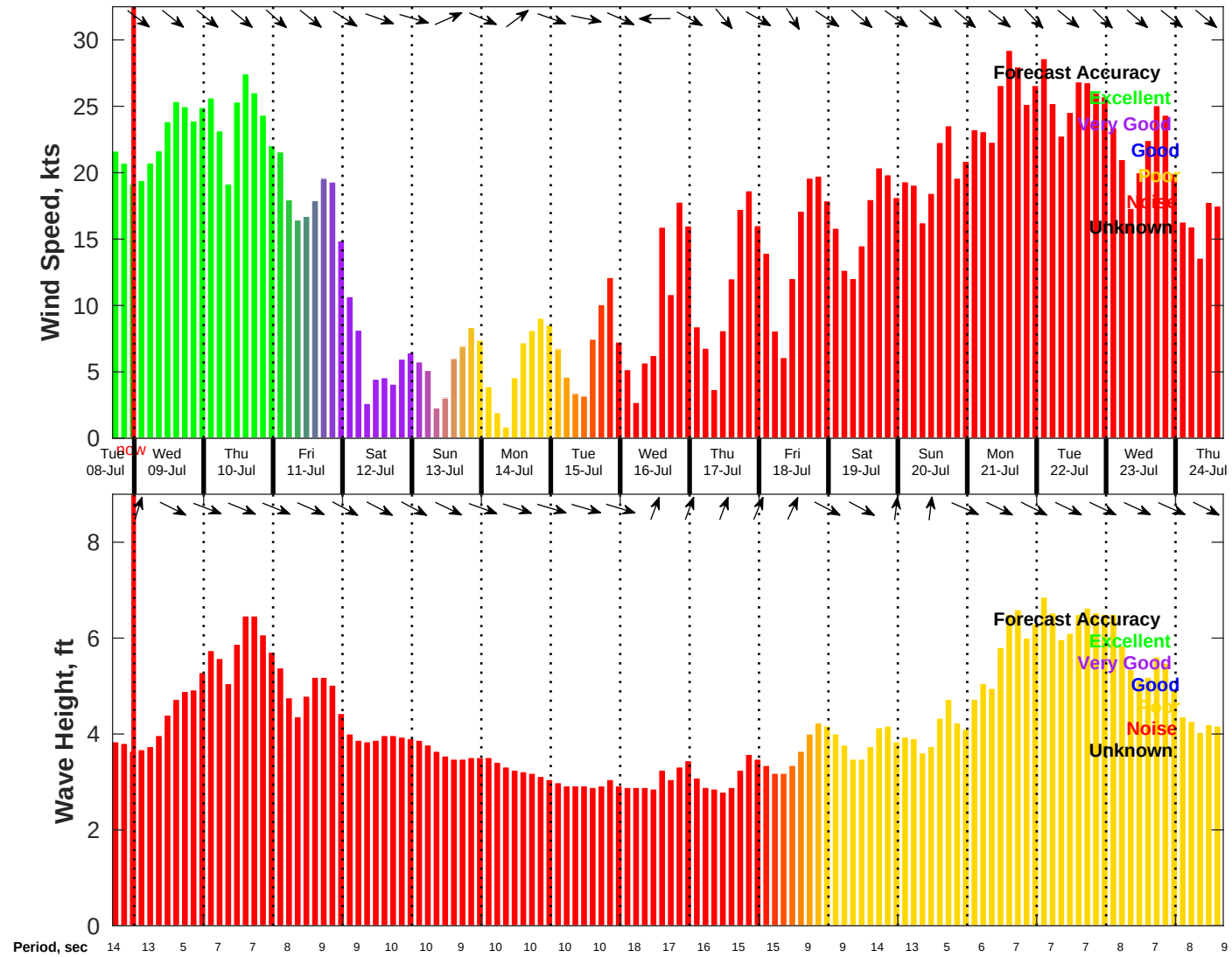
Wind & Wave Forecast for NDBC 46054 from 08-Jul-2025 16:00:00 to 24-Jul-2025 16:00:00
