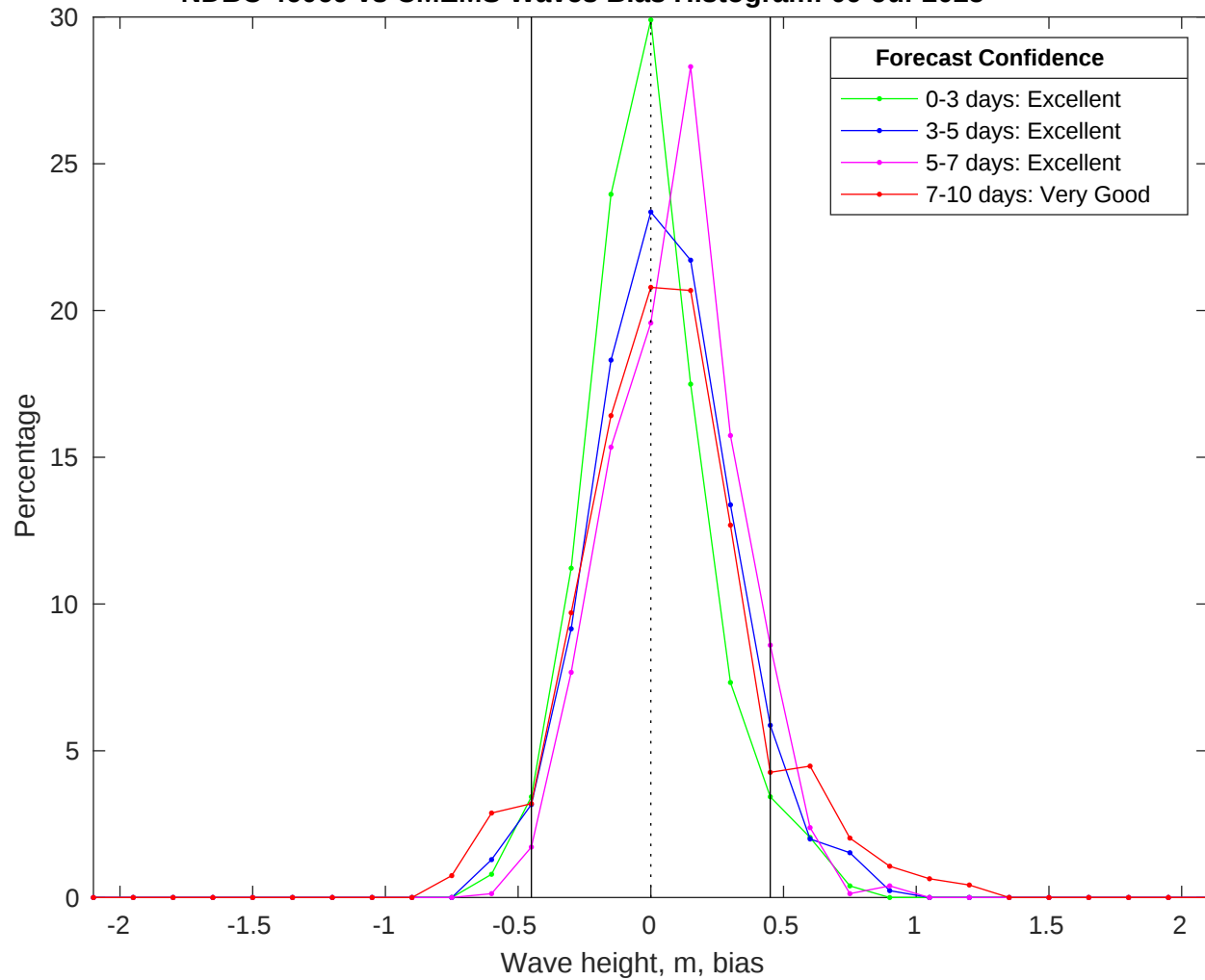
NDBC 46069 vs CMEMS Waves Bias Histogram: 09-Jul-2025
