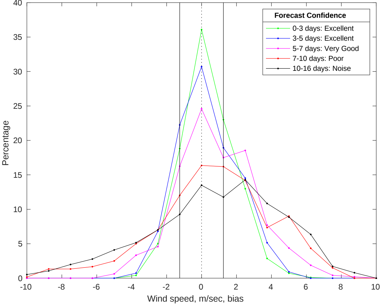
NDBC 46069 vs GFS Winds Bias Histogram: 09-Jul-2025
