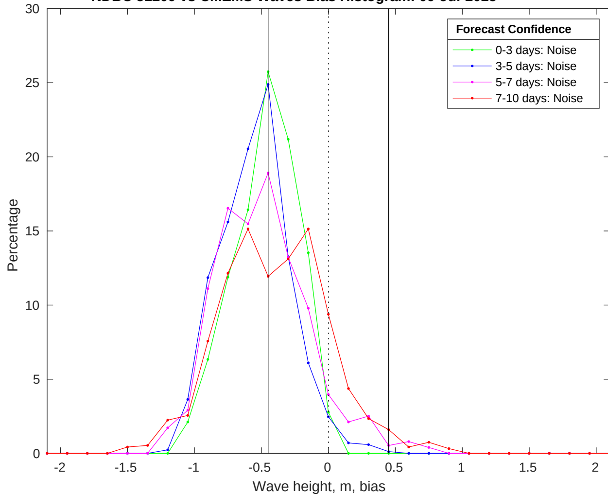
NDBC 51209 vs CMEMS Waves Bias Histogram: 09-Jul-2025
