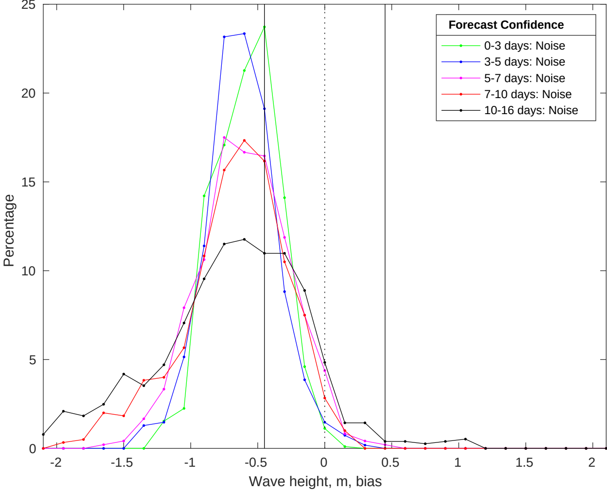
NDBC 51209 vs GFS Waves Bias Histogram: 09-Jul-2025
