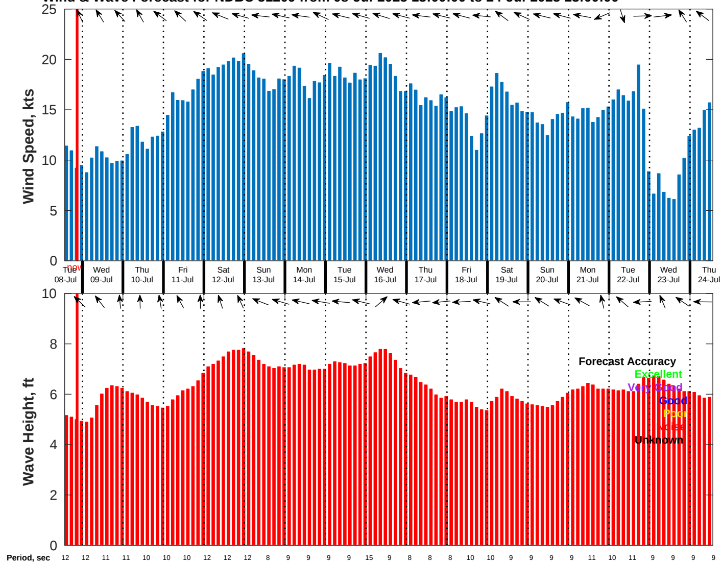
Wind & Wave Forecast for NDBC 51209 from 08-Jul-2025 13:00:00 to 24-Jul-2025 13:00:00
