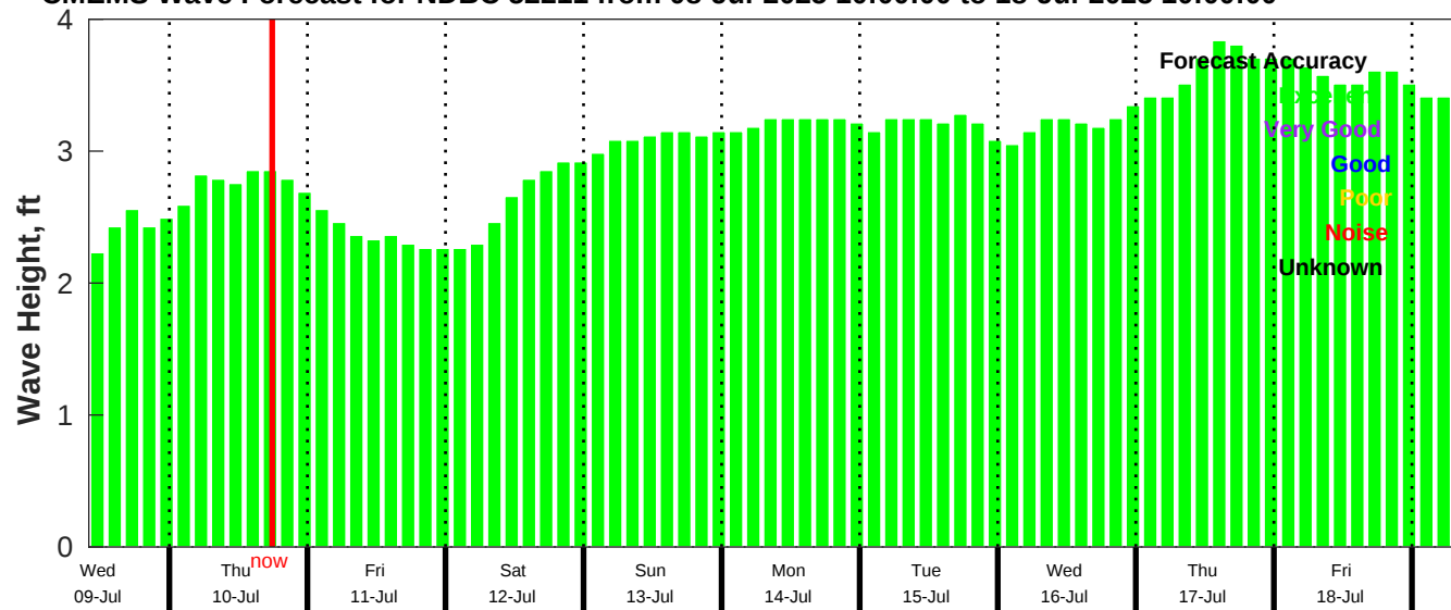
CMEMS Wave Forecast for NDBC 52211 from 08-Jul-2025 10:00:00 to 18-Jul-2025 10:00:00
