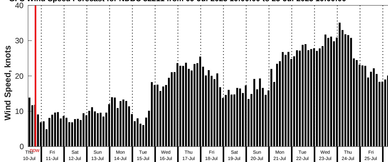
GFS Wind Speed Forecast for NDBC 52211 from 09-Jul-2025 10:00:00 to 25-Jul-2025 10:00:00
