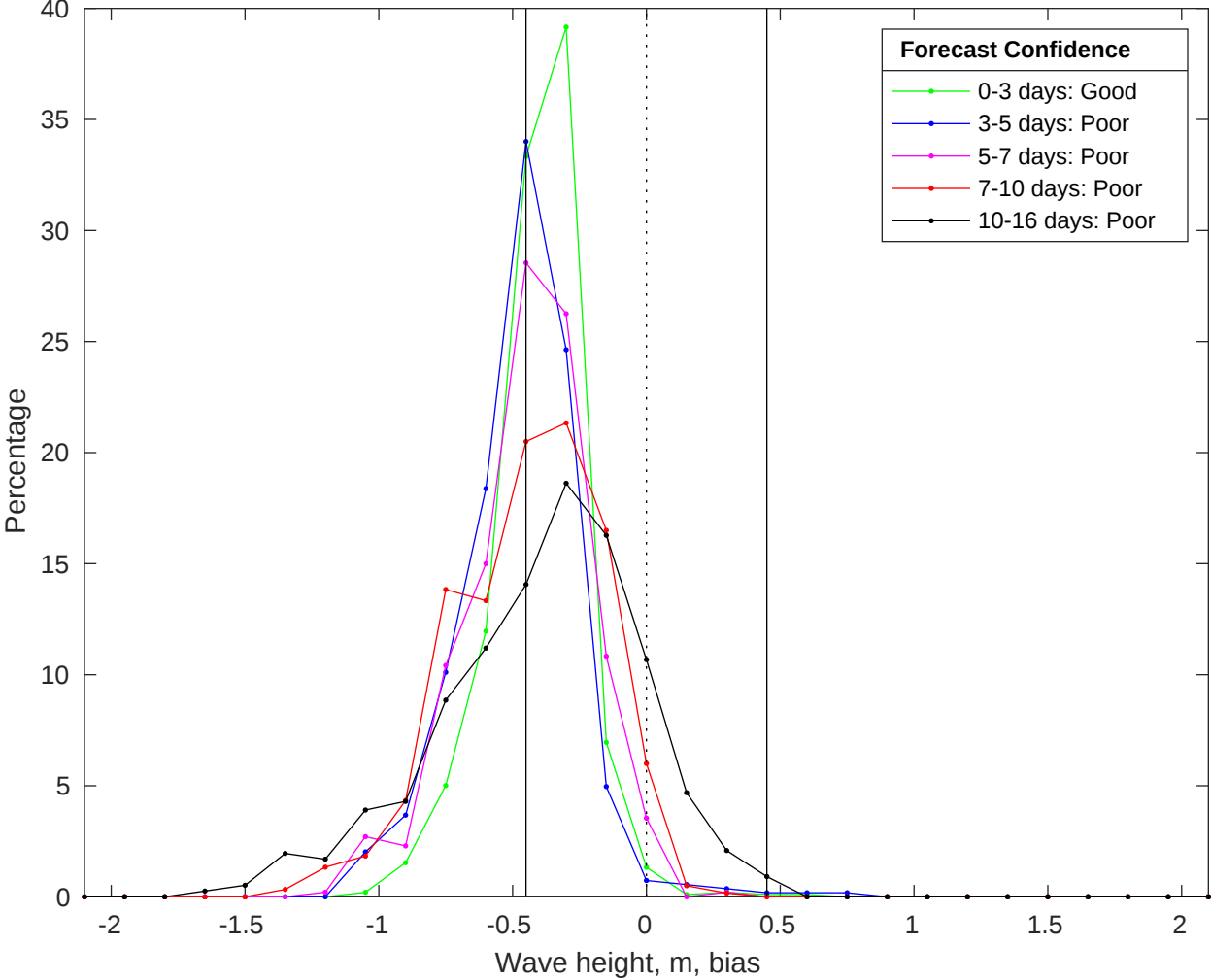
NDBC 52213 vs GFS Waves Bias Histogram: 09-Jul-2025
