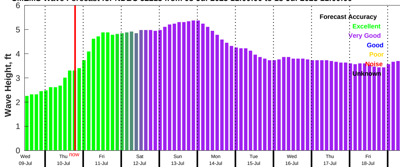
CMEMS Wave Forecast for NDBC 52213 from 08-Jul-2025 11:00:00 to 18-Jul-2025 11:00:00
