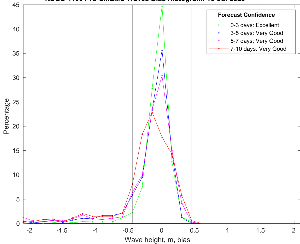
NDBC 41004 vs CMEMS Waves Bias Histogram: 10-Jul-2025
