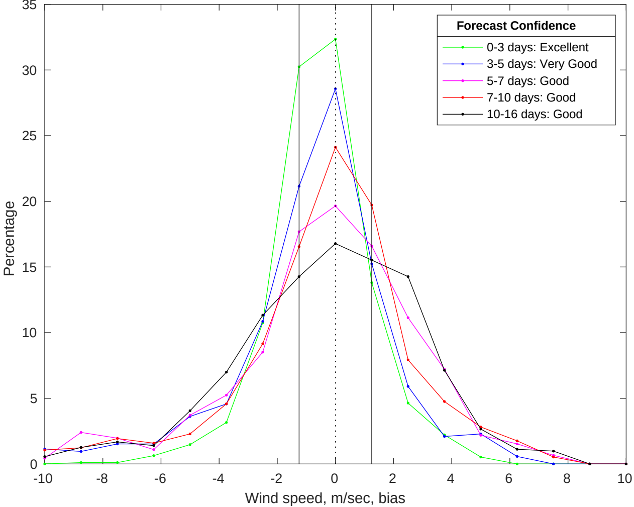
NDBC 41004 vs GFS Winds Bias Histogram: 10-Jul-2025
