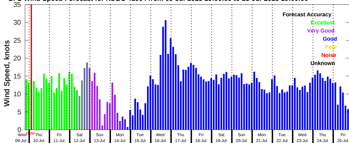
GFS Wind Speed Forecast for NDBC 41004 from 09-Jul-2025 19:00:00 to 25-Jul-2025 19:00:00
