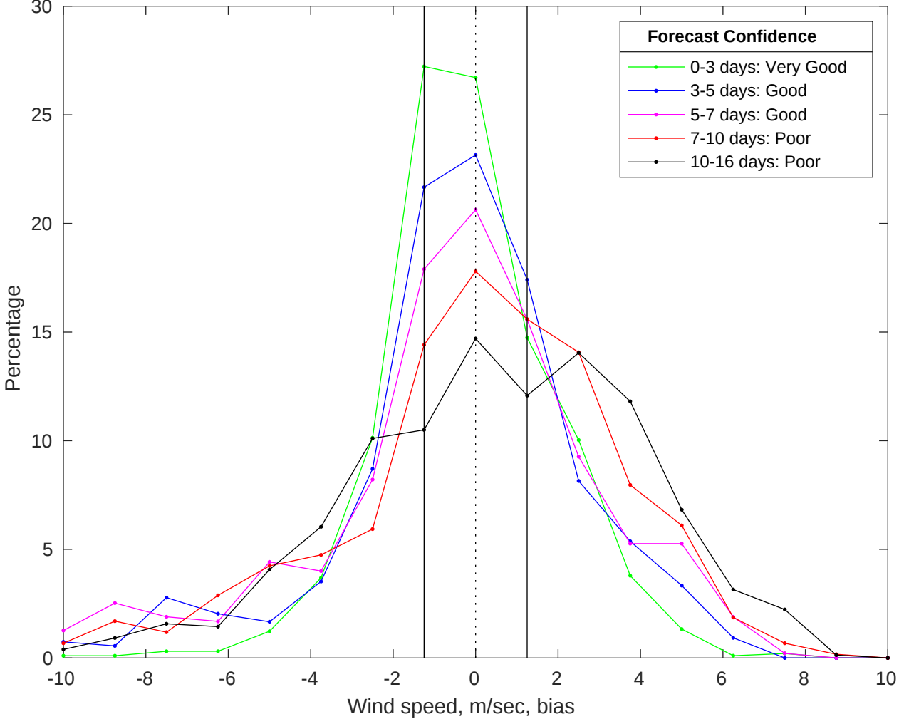
NDBC 41013 vs GFS Winds Bias Histogram: 10-Jul-2025
