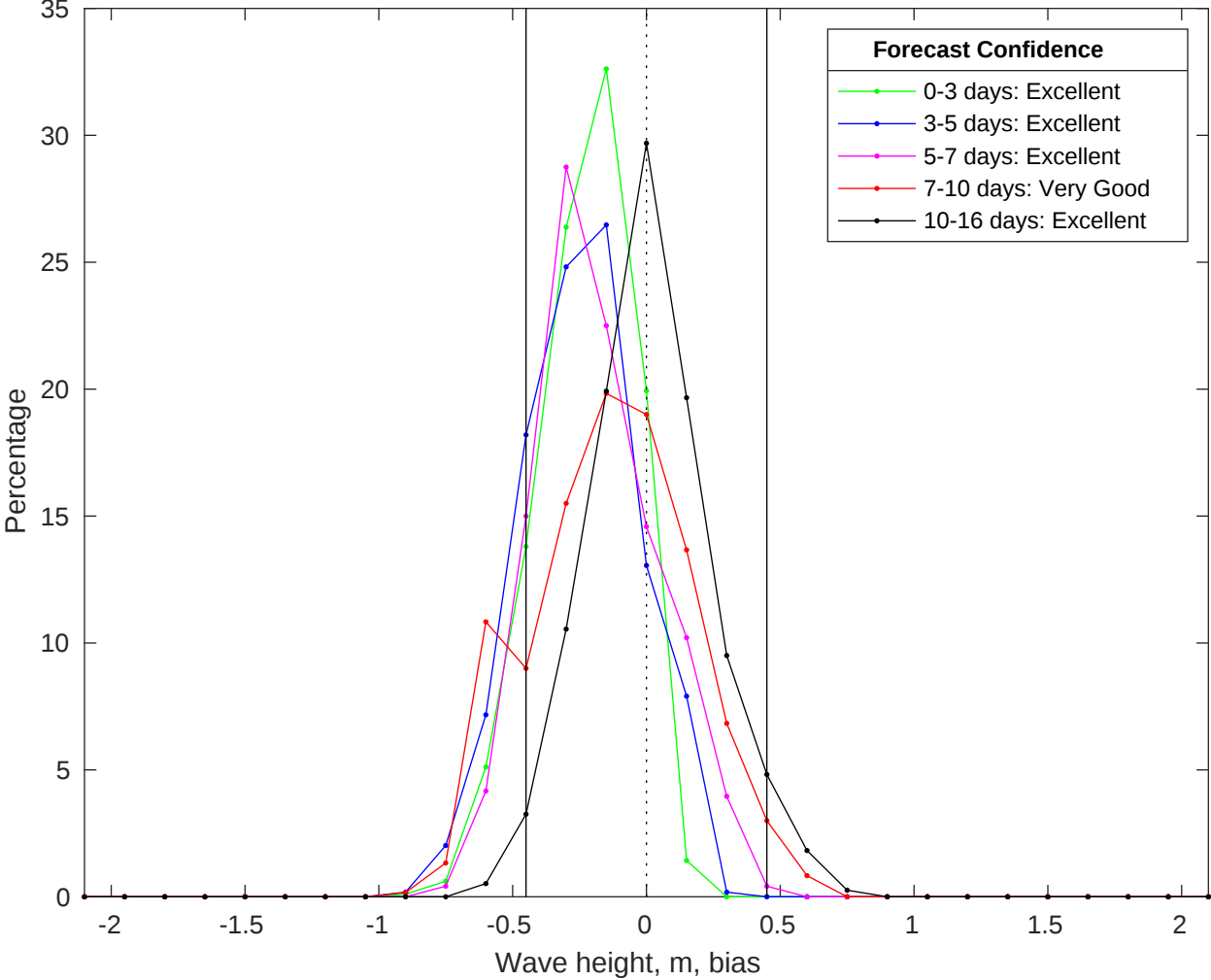
NDBC 41040 vs GFS Waves Bias Histogram: 10-Jul-2025
