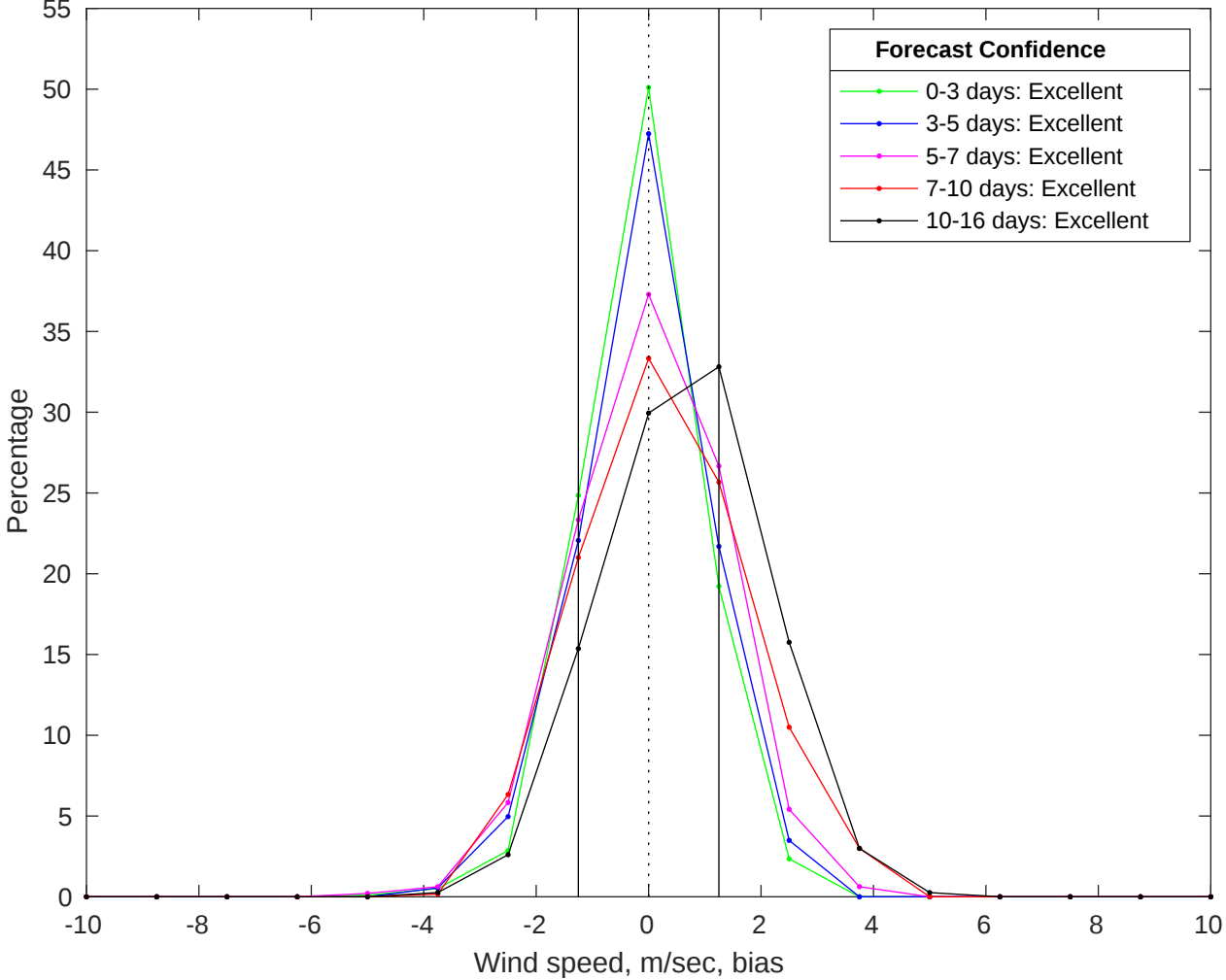
NDBC 41040 vs GFS Winds Bias Histogram: 10-Jul-2025
