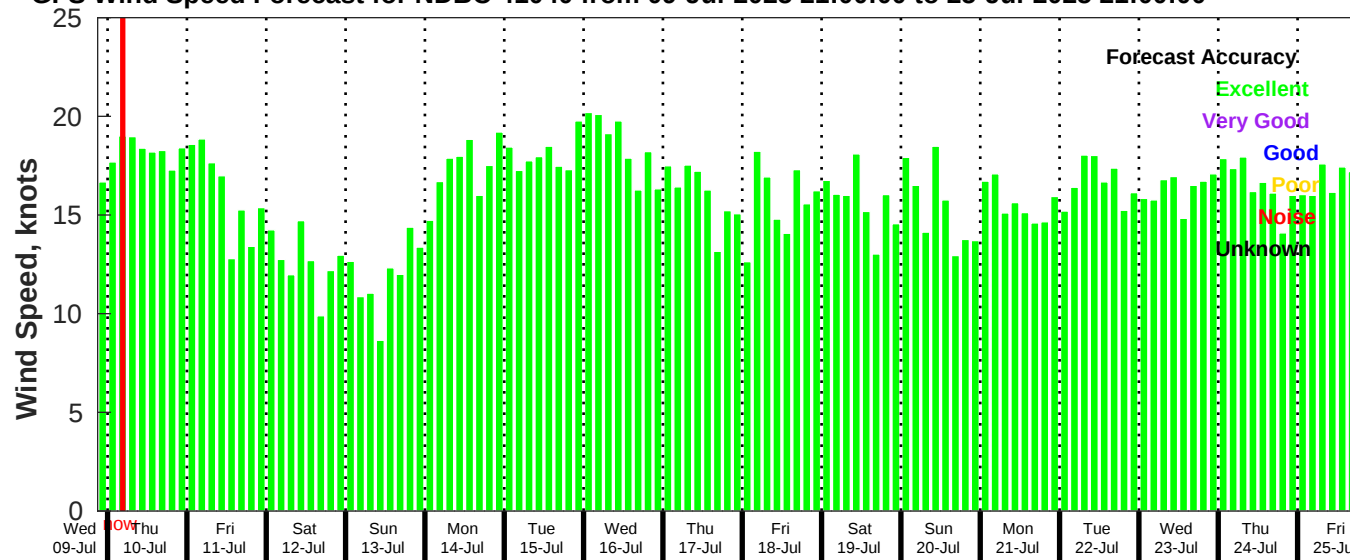
GFS Wind Speed Forecast for NDBC 41040 from 09-Jul-2025 21:00:00 to 25-Jul-2025 21:00:00
